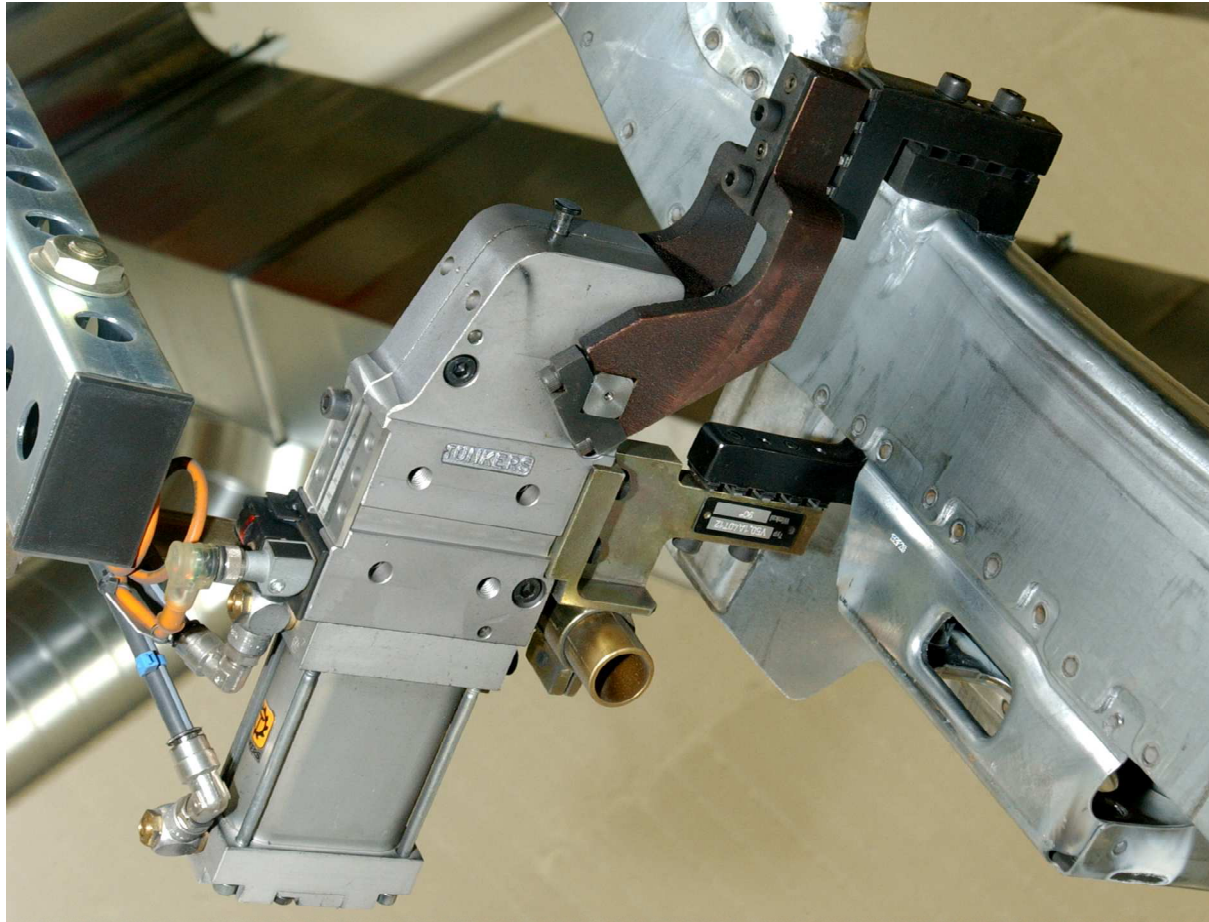
Vario series – Pneumatic clamps for line production in the body assembly
